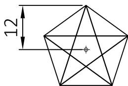
Inscribed Pentagon
