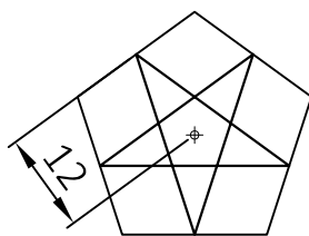
circumscribed pentagon
